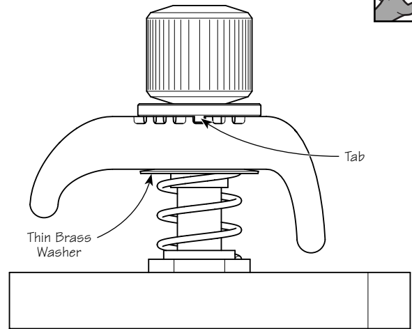
Figure 6: Adding the clamp arms. Note orientation of the thin brass washer.
