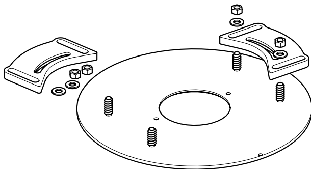
Figure 2: Removing the clamp bases.
