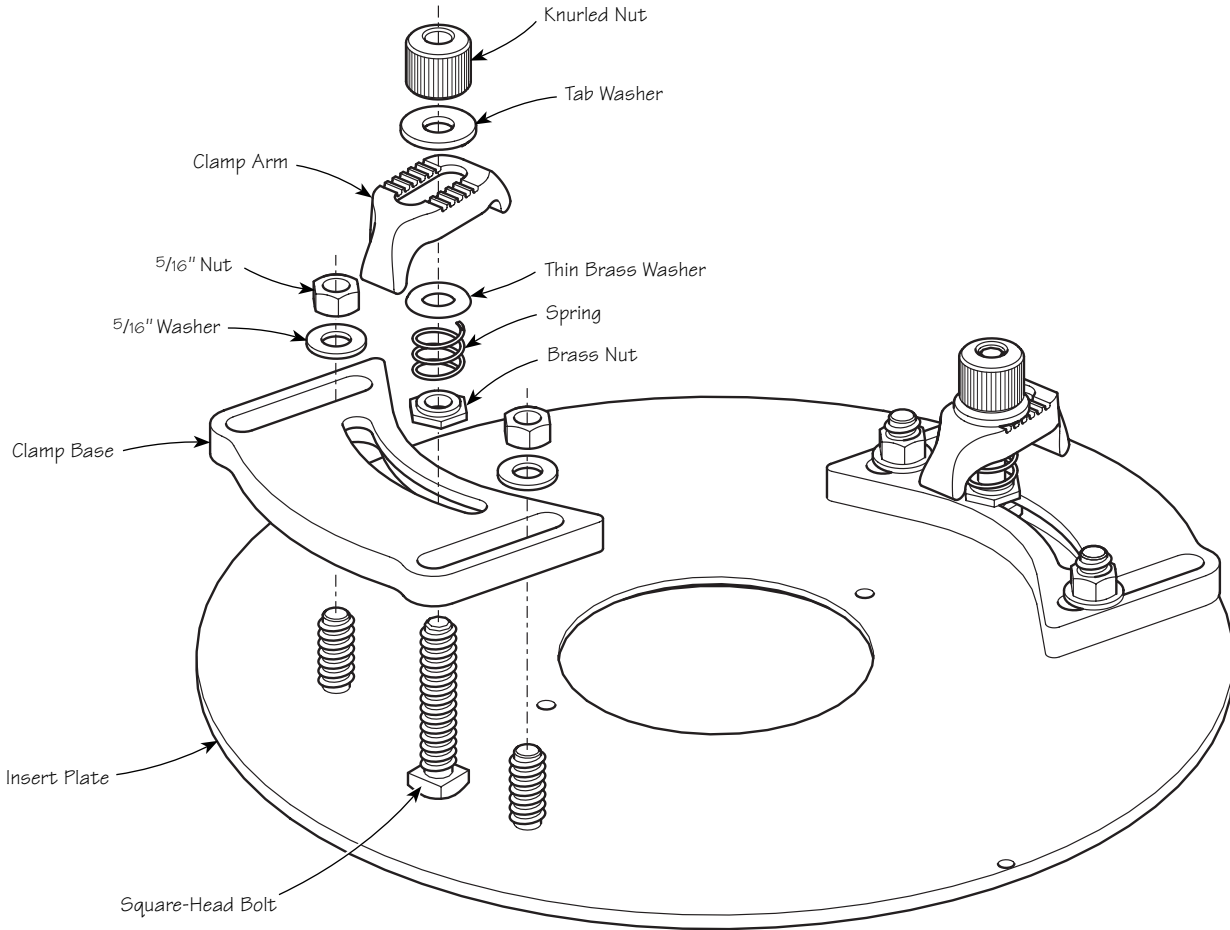
Figure 1: Components of the router table insert plate.
