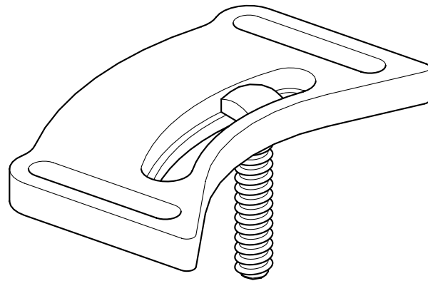
Figure 3: Inserting the square-head bolt into the clamp base.
